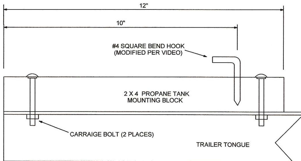
PROPANE TANK MOUNTING BLOCK DETAIL CUTAWAY VIEW
